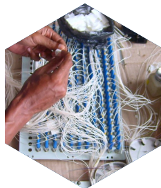
FIBER TERMINATION (OTB)
